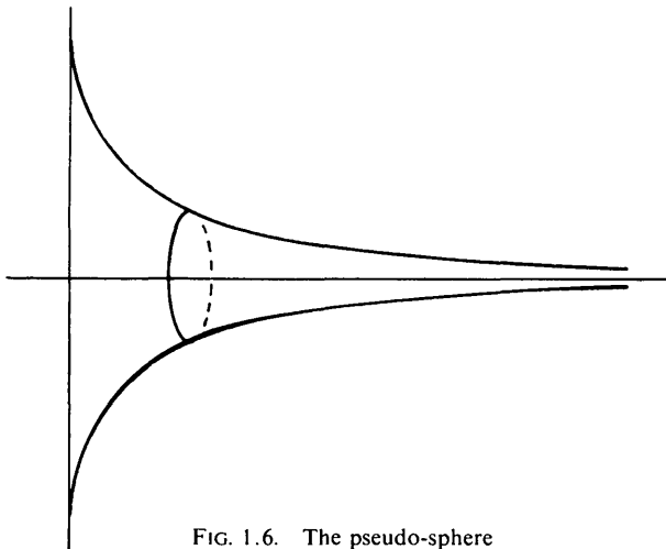
FIG. 1.6. The pseudo-sphere
