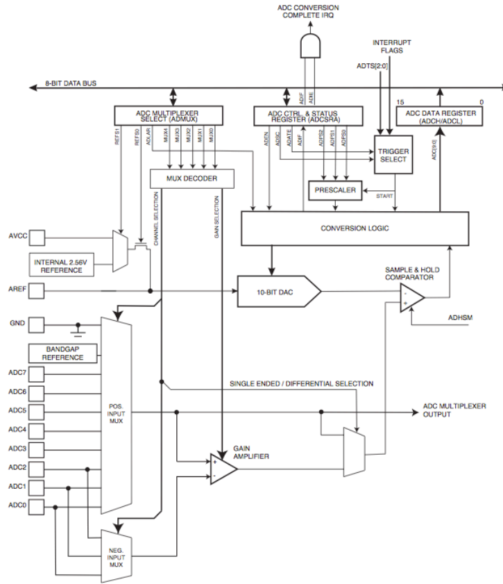
Figure 98. Analog to Digital Converter Block Schematic
